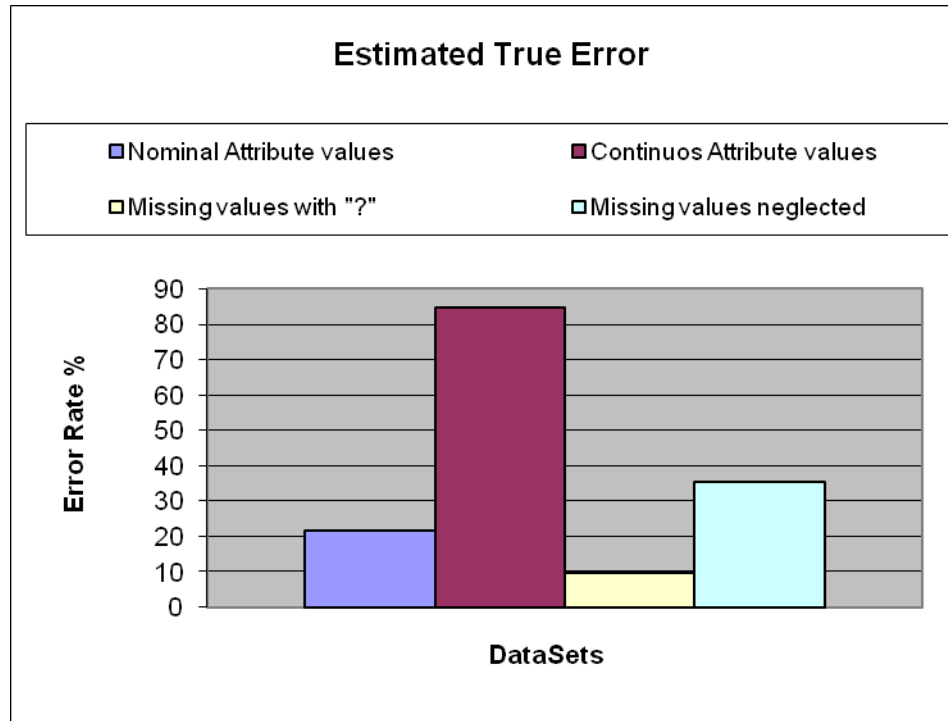
Figure 2. Performance of ID3
