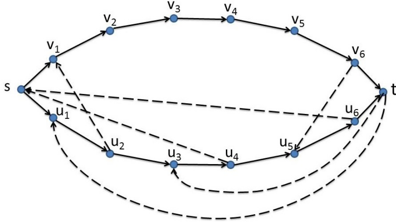
Fig. 4. An example of a graph which does not have a reverse-compatible optimum solution for 2-SCSS-(2, 2).
